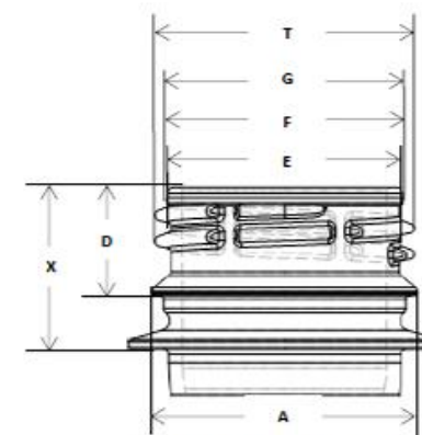
Rosca Baja PCO 1881 – 28mm
