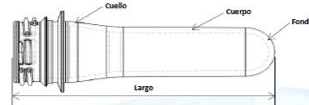
Rosca Baja PCO 1881 – 28mm
